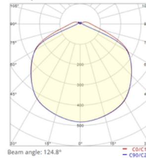
Polar plot
