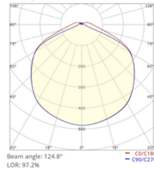
Polar plot
