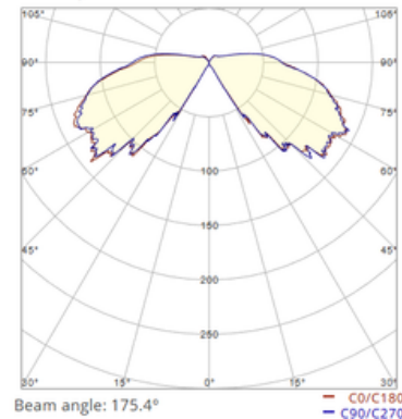
Polar plot
